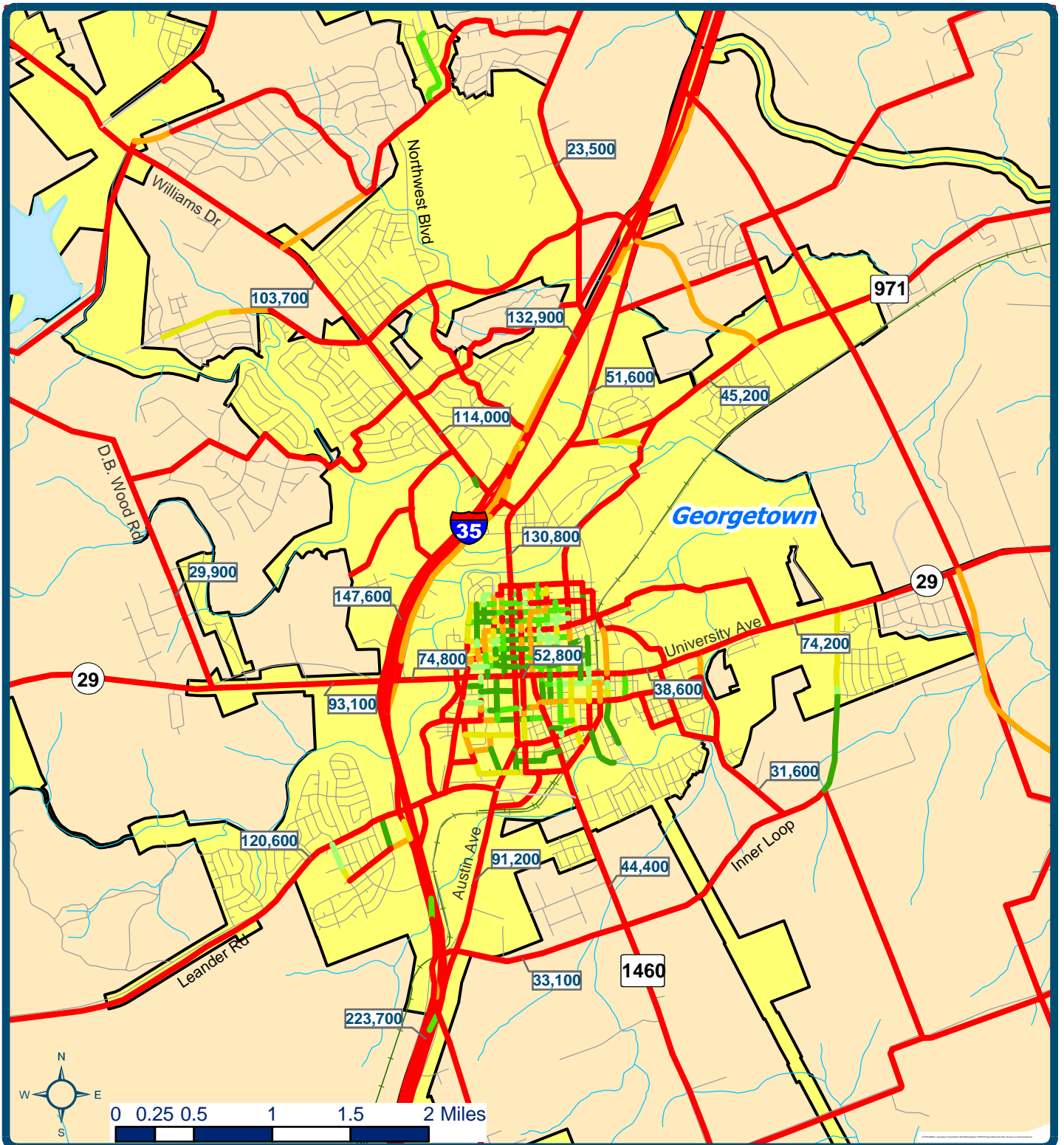
Figure 5-2b (Inset) Year 2030 Projected Daily Traffic Volumes and Level of Service (No Build Plus Under Construction Network) Georgetown Overall Transportation Plan Georgetown, TX
