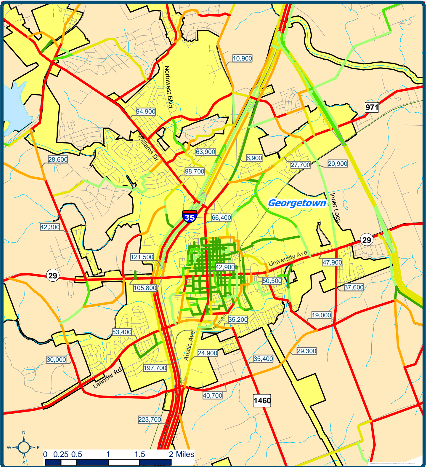
Figure 5-4b (Inset) Year 2030 Projected Daily Traffic Volumes and Level of Service (GTEC Existing Plus Committed Network)
