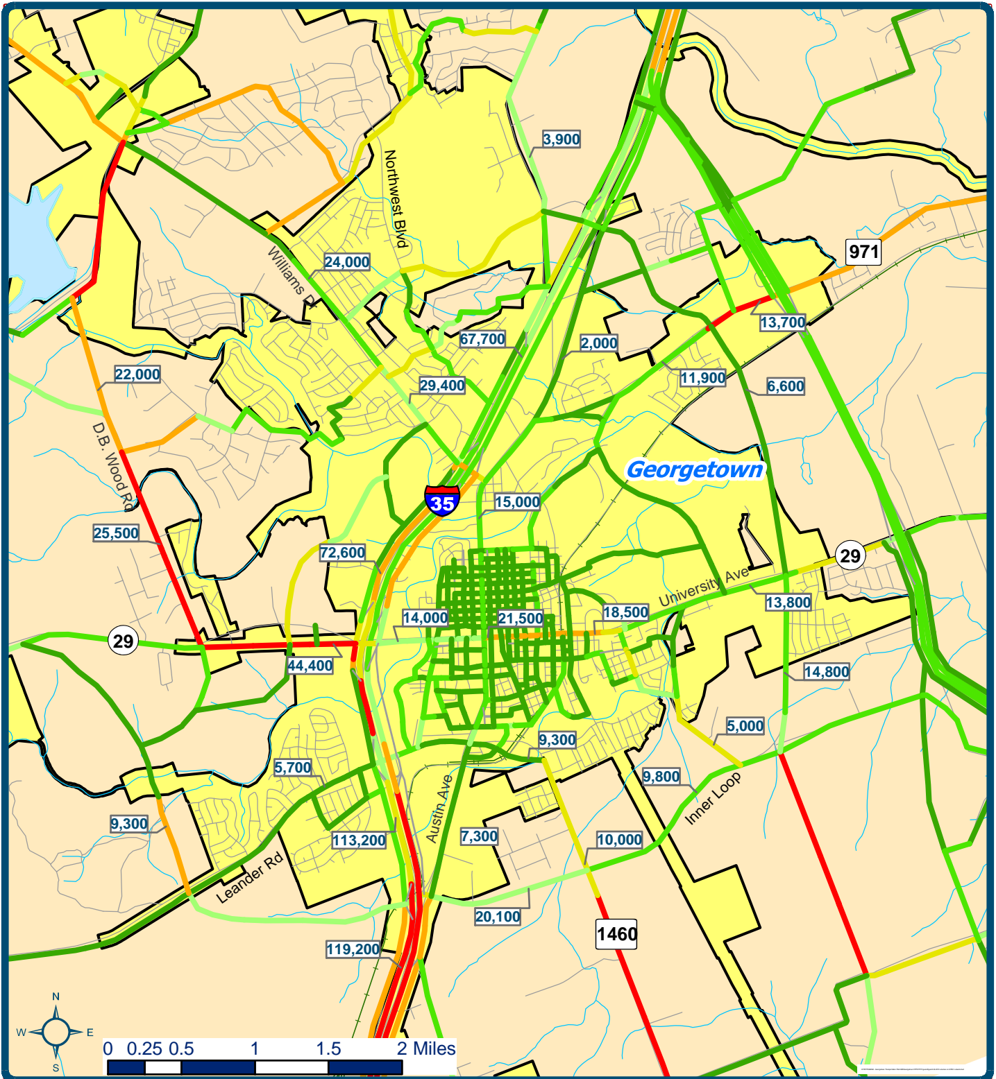
Figure 5-3b (Inset) Year 2010 Projected Daily Traffic Volumes and Level of Service (GTEC Existing Plus Committed Network)
