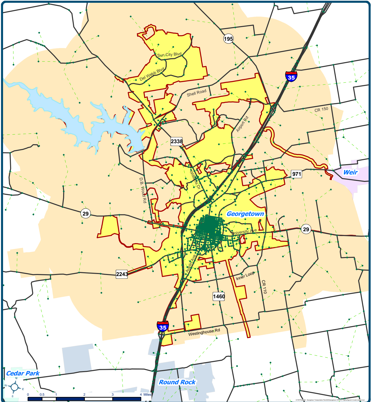
Figure 3-3 Travel Model Network Links and Nodes
